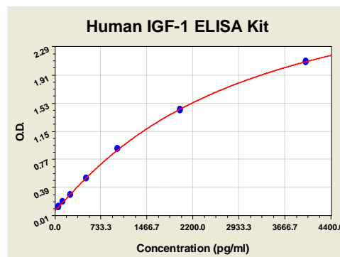
Figure 1: IGF-1 Standard Curve. Using the Human IGF-1 ELISA Kit, O.D. data was graphed against IGF-1 protein concentration. The TMB reaction was incubated at 37°C for 27 min.
